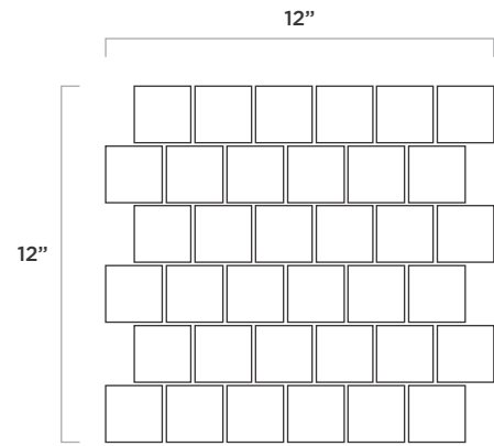
2"x2" OFFSET MOSAIC
